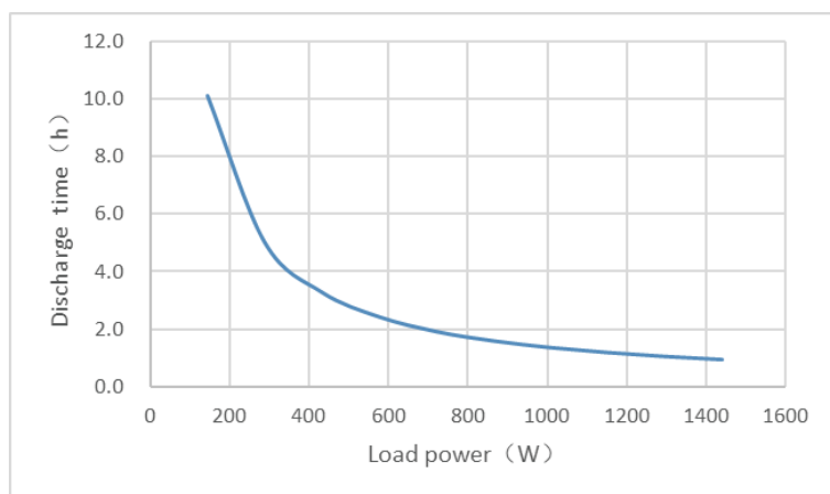
SDA10-4830 Discharge time at different load power
